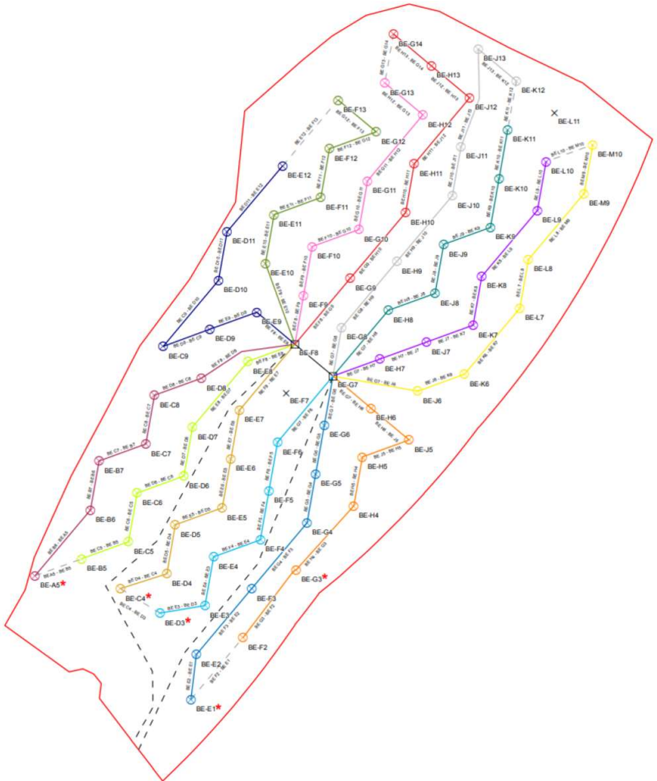
Figure 1- Array Cable Routes for Survey (Scope E)
