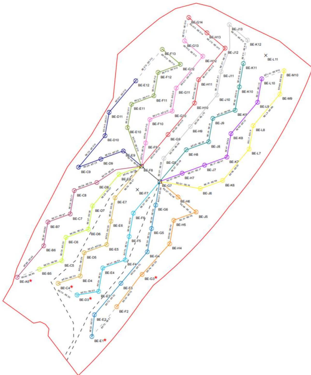
Figure 1- Array Cable Routes for Survey (Scope E)
